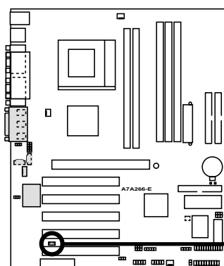
A7A266-E Wake-On-LAN Connector
